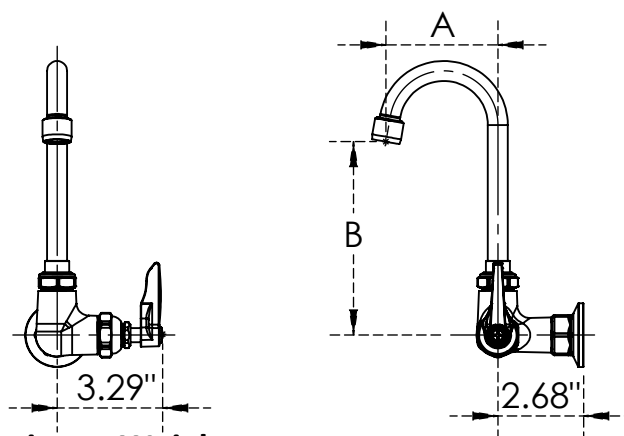
Dimensions - Weights
